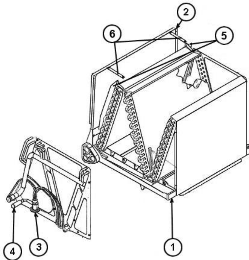
Coil Assembly
