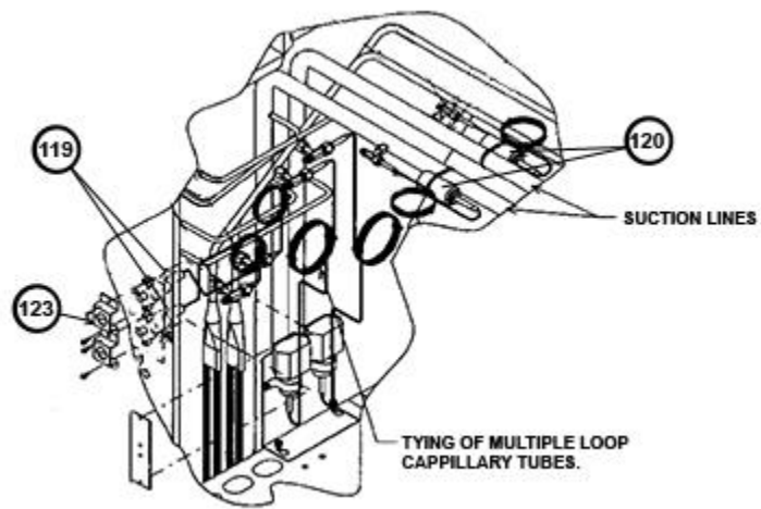
RXRX-AK01 General Assembly
