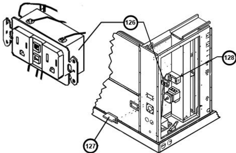
RXRX-AN01 Assembly
