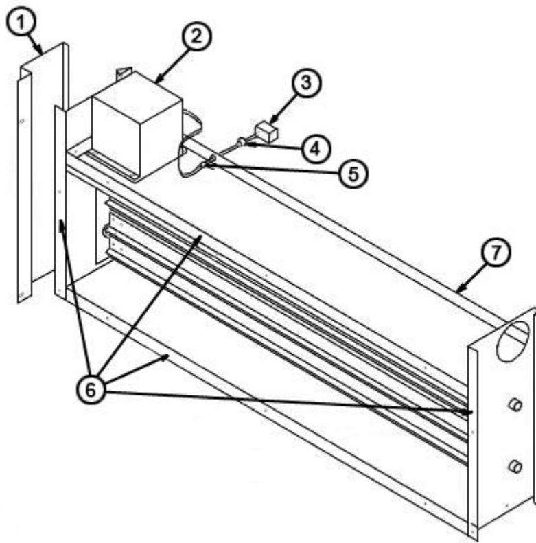
RXRX-AT02 Assembly
