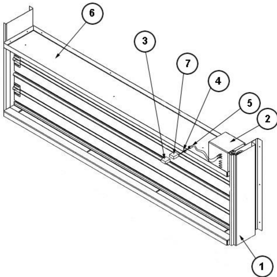
RXRX-AW03 Assembly
