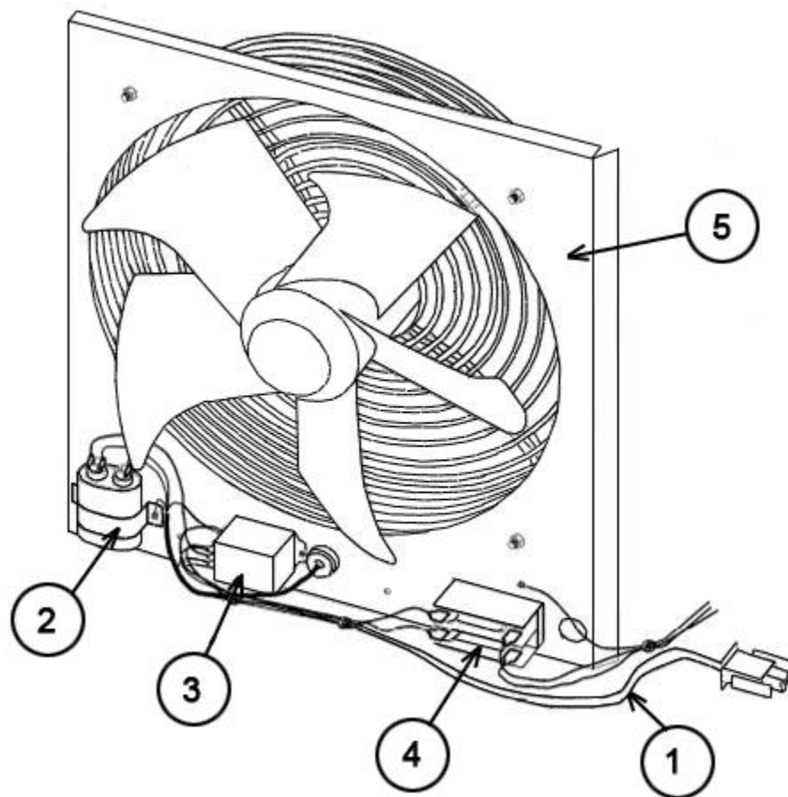
RXRX-BFF04C Assembly
