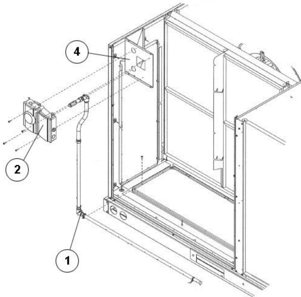
RXRX-BS02 (1) Assembly
