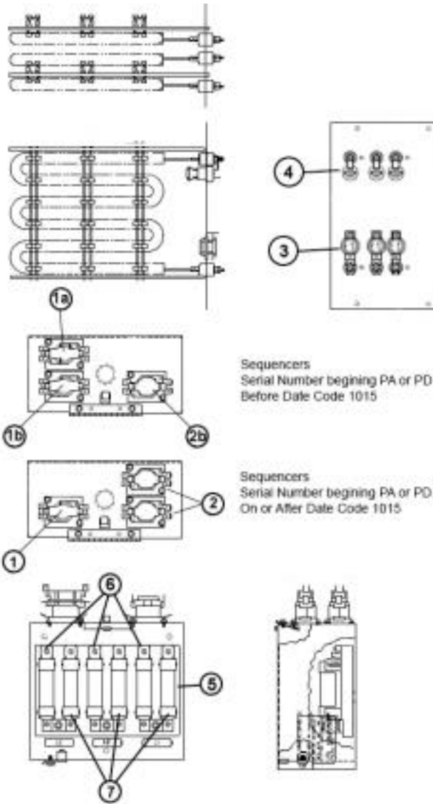
Drawing of RXQJ C015C
