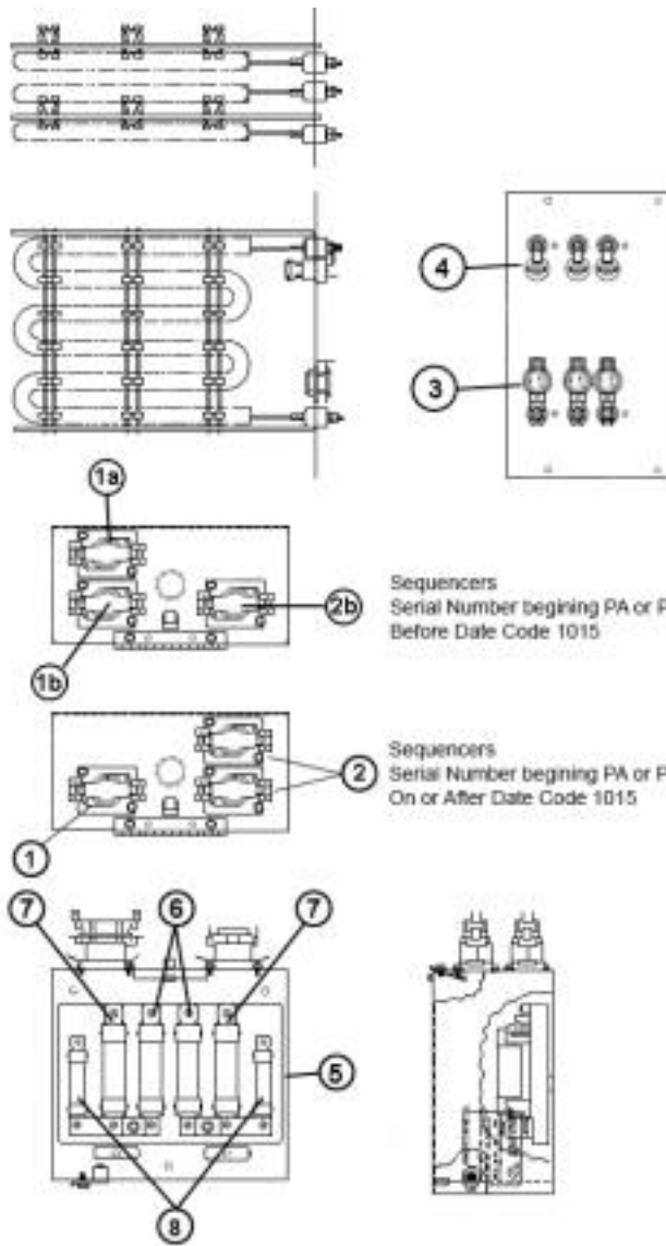
Drawing of RXQJ C015J
