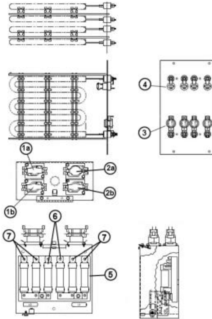
Drawing of RXQJ C020J
